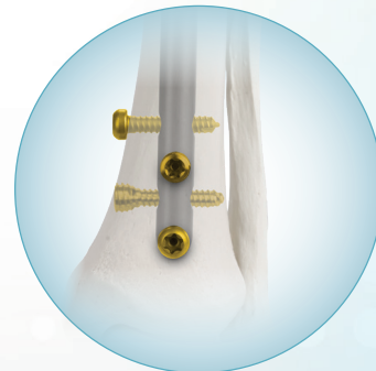
Headless locking screw option
