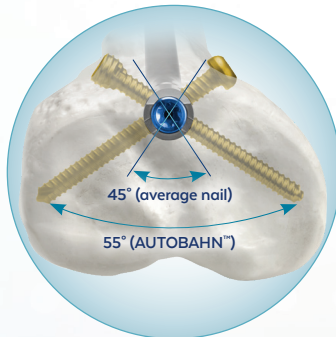
55° proximal oblique screw angle
